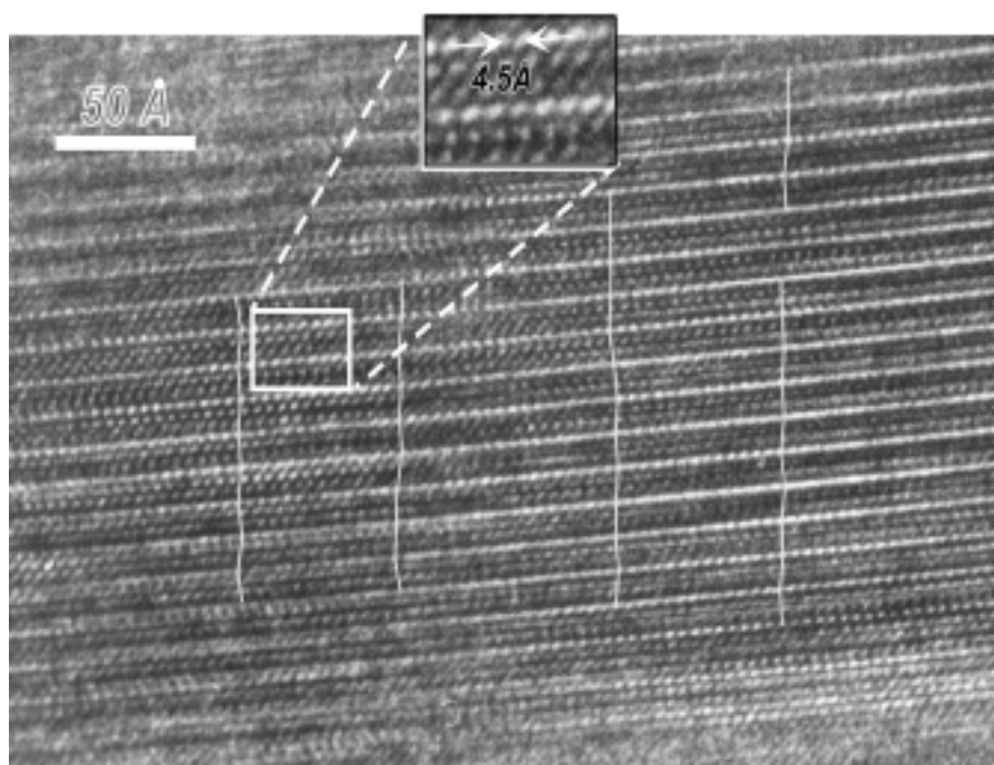
Figure 4.—Lattice fringe image of illite and I-S in the studied sample. The cross-fringes demonstrate the coherence of the stacked layers. Because of the 4.5 \text{ \AA} spacing in the bright strip (AHN and BUSEK, 1990) and by analogy with images of AMOURIC et al. (1981), the view must be along [1 \ 1 \ 0] or [1 \ 1 \ 0] of a 2M_1 polytype. This ordering appears to be disturbed laterally by comparing the stack sequence (white breaks in the lines) and some defects may occur. The brighter spots are attributed to smectite interlayers.
