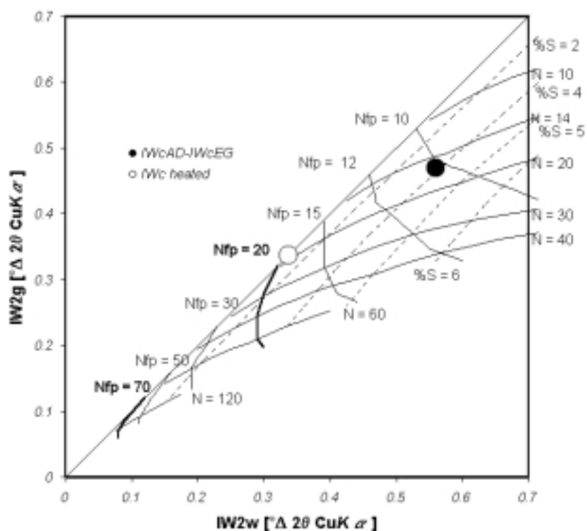
Figure 1.—Plot of illite width corrected ( IW_c ) for I-S containing 2 water planes ( IW_{2w} ) versus IW_c for I-S containing 2 ethylene-glycol interlayers ( IW_{2g} ), assuming R = 1 ordering (JABOYEDOFF et al. 2001). The black spot represents the IW_{cAD} and IW_{cEG} values for the studied sample and the white spot represents the IW_c for a heated sample, assuming that heated specimen is equivalent to 0% S and N is then determined using IW_{2w} = IW_{2g} . Anchizone limits without instrumental effect are 0.10^\circ and 0.30^\circ 2\theta \text{CuK}\alpha .
